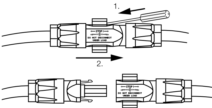
Fig. 37: Desligar o conector SUNCLIX
