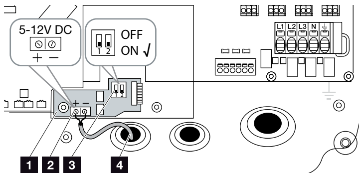
Fig. 26: Placa KOSTAL Smart AC Switch
