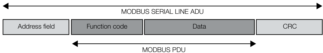
Abb. 9: MODBUS frame Serial Line
