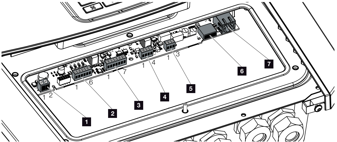
Afb. 26: Smart Communication Board - interfaces
