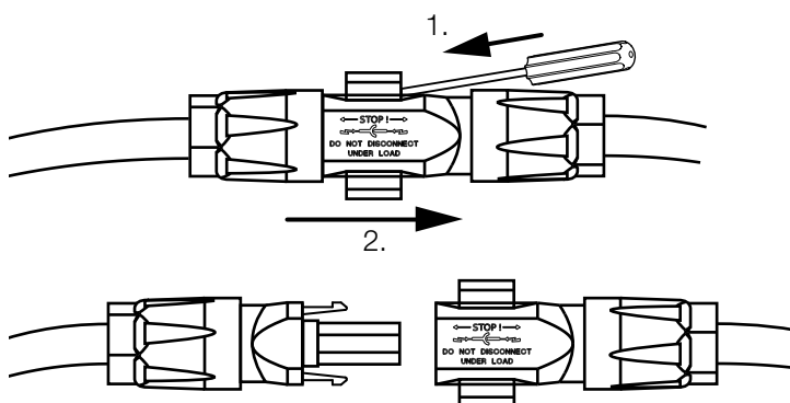
Afb. 41: SUNCLIX DC-stekkers loskoppelen
