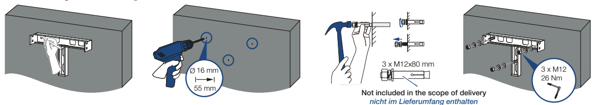
Wall mounting / Wandmontage
